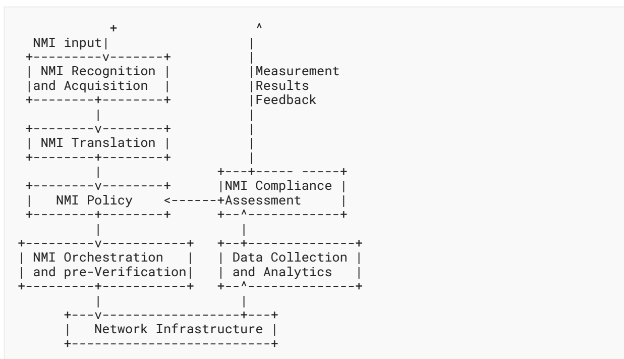
Figure 1: Full Lifecycle of NMI
