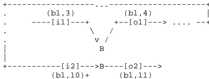
Fig.12 Load splitting at intermediate node
