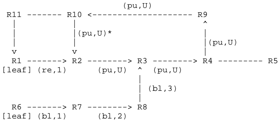
Fig.15 The network state
