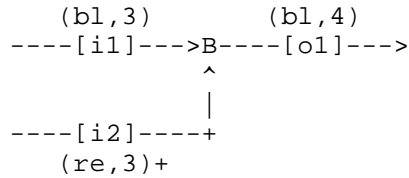
Fig.5 Thread merging
