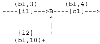
Fig.6 Thread stalling (1)
