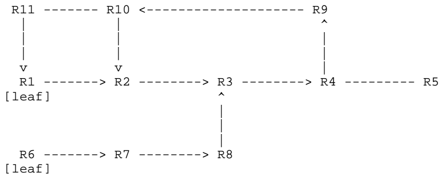
Fig. 14 Example MPLS network (1)
