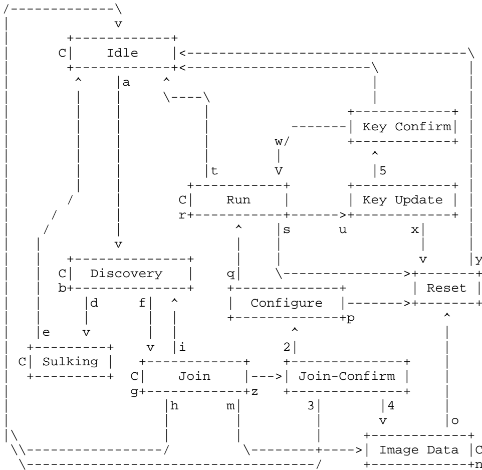
Figure 2: LWAPP State Machine
