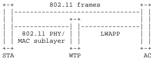
Figure 1: LWAPP Architecture
