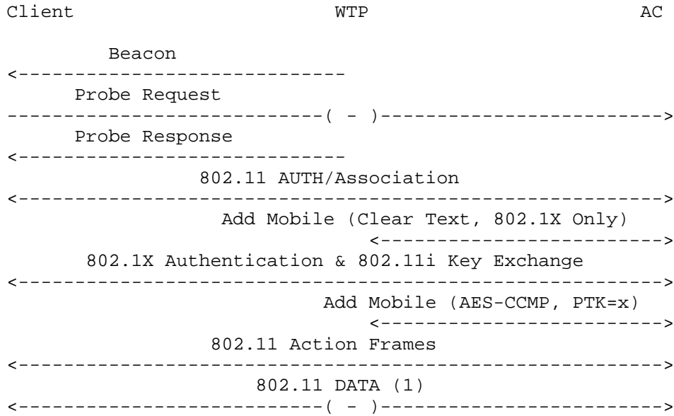
Figure 4: Split MAC Message Flow
