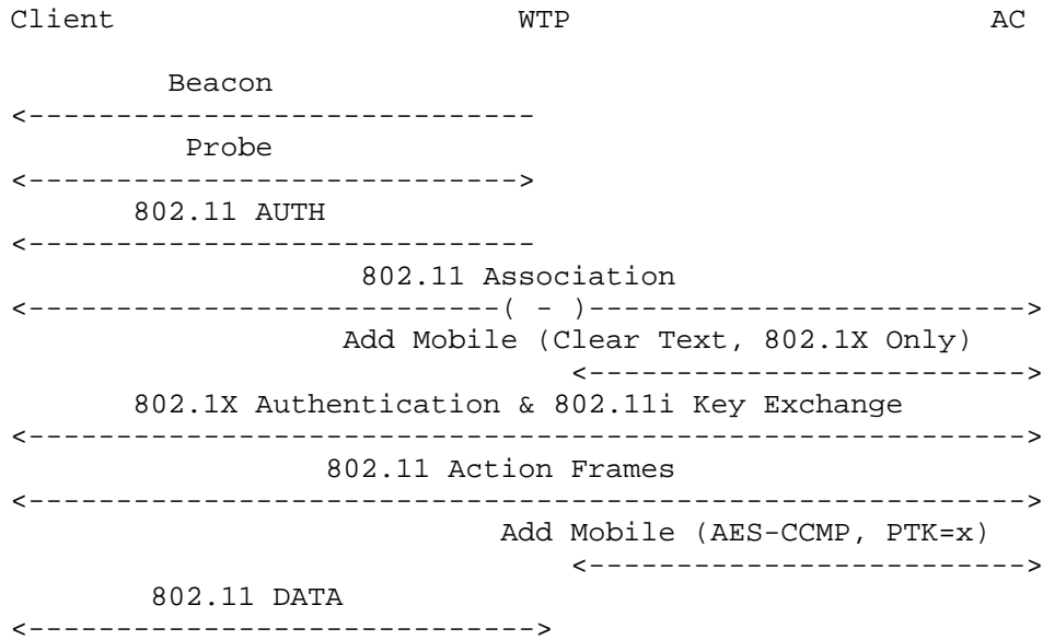
Figure 6: Local MAC Message Flow
