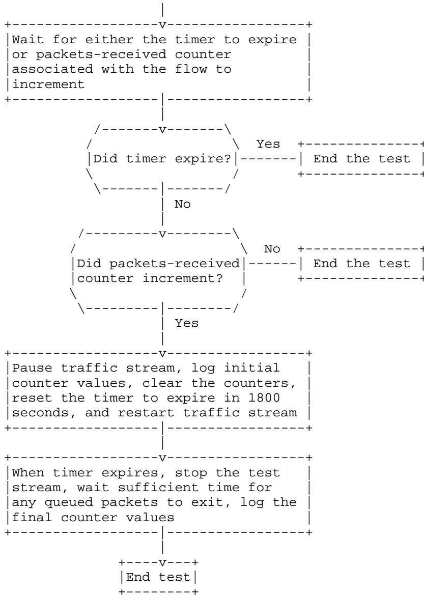
Figure 2: Baseline Test Procedure Flow Chart
