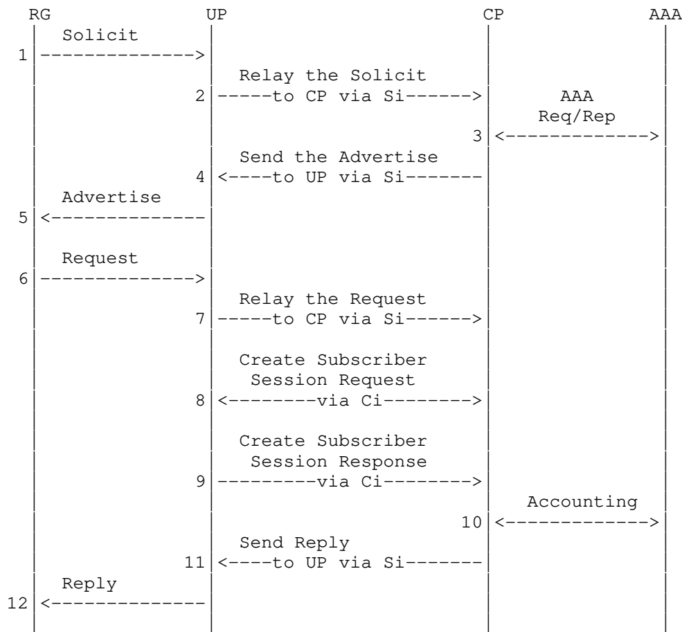
Figure 15: DHCPv6 Access
