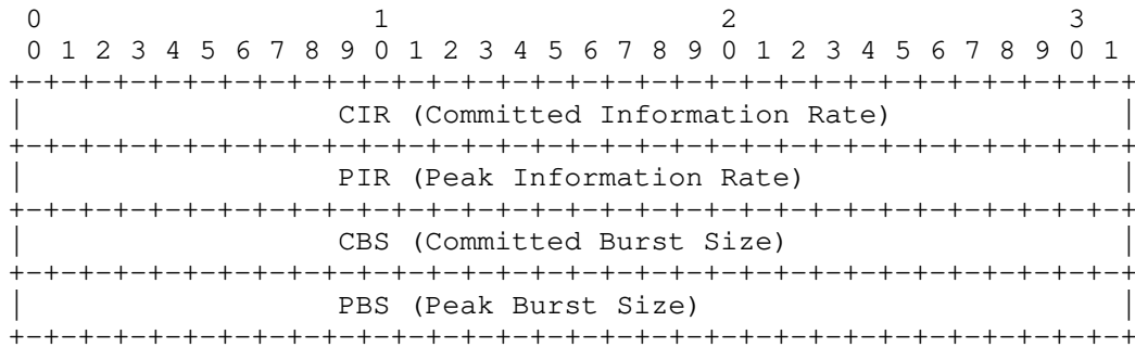
Figure 35: Egress-CAR Sub-TLV
