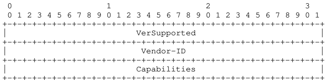
Figure 39: Hello TLV
