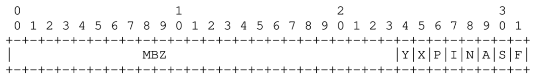
Figure 43: Interface Flags
