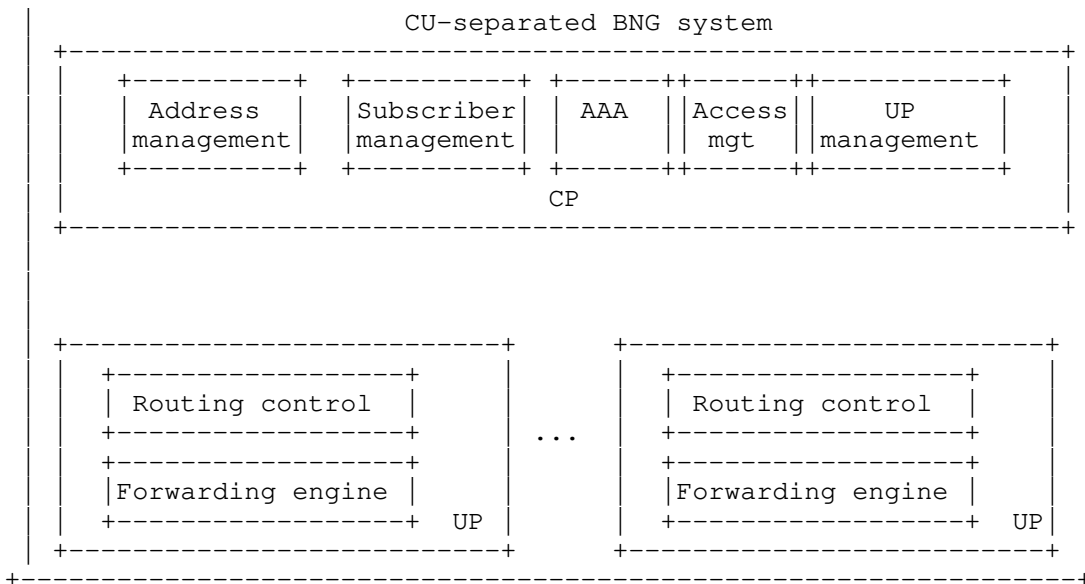
Figure 1: Architecture of a CU-Separated BNG
