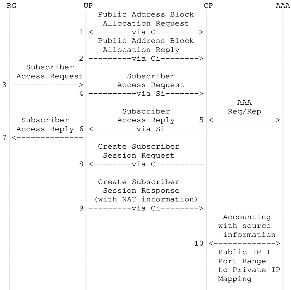
Figure 27: CGN Access
