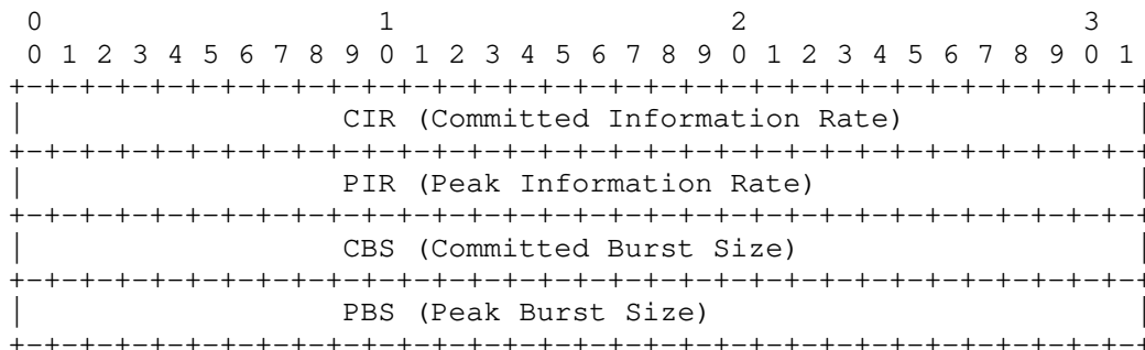
Figure 34: Ingress-CAR Sub-TLV
