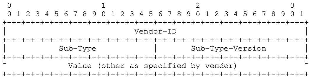
Figure 38: Vendor Sub-TLV
