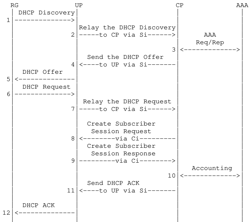
Figure 14: DHCPv4 Access
