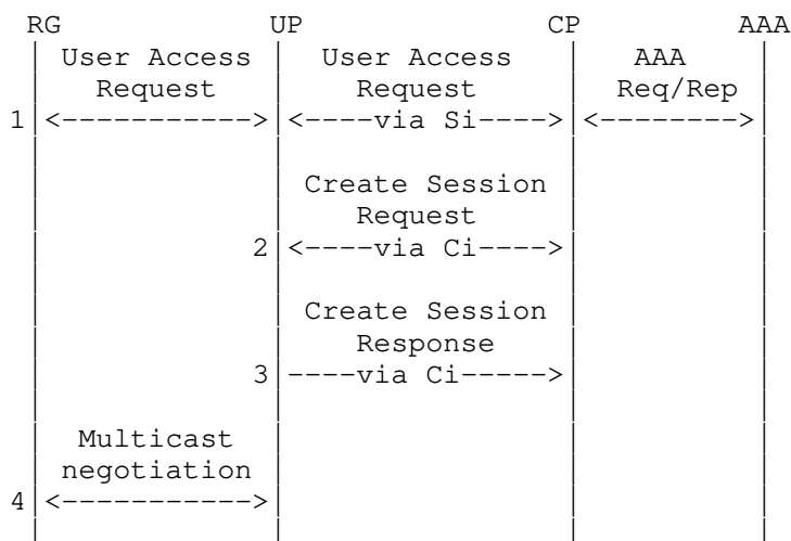
Figure 30: Multicast Access
