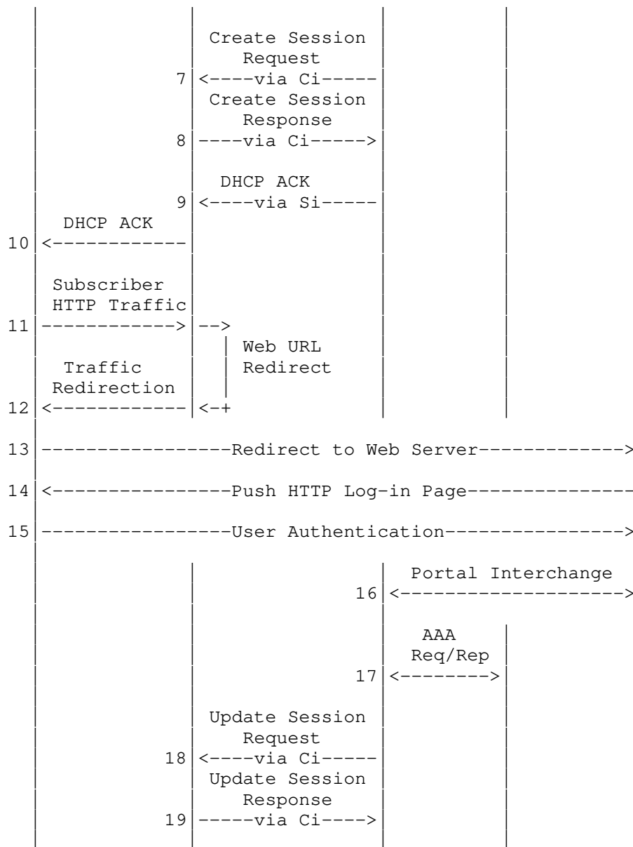
Figure 23: WLAN Access
